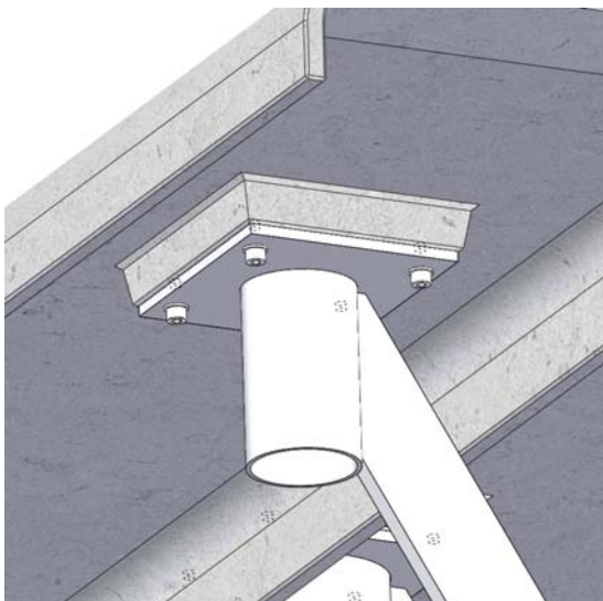
Detail 1: seat fixing
